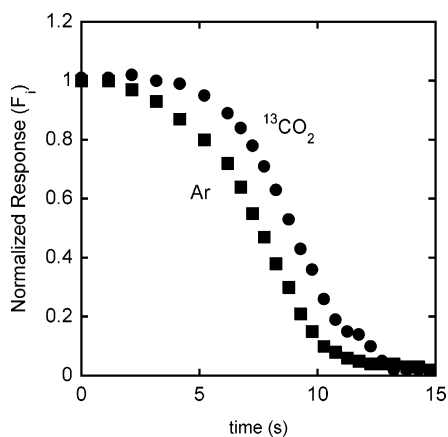
Figure 1. Example of an isotopic transient during CO oxidation over CsX at 573 K.
